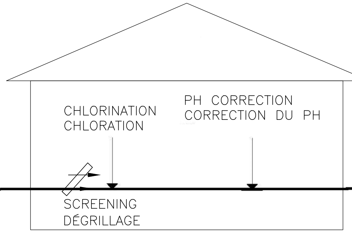
EXISTING FACILITIES INSTALLATIONS EXISTANTES
